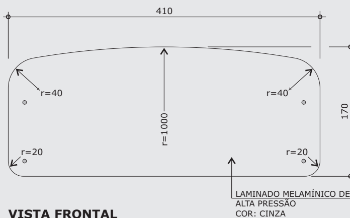
VISTA FRONTAL
